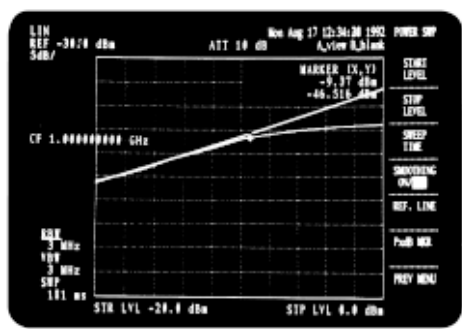
Amplifier 1 dB gain compression point measurement
